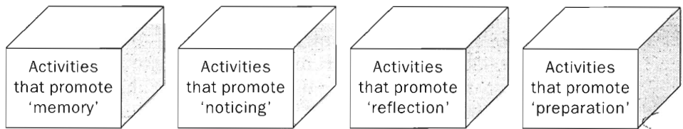
Figure 6.5 Additional blocks
