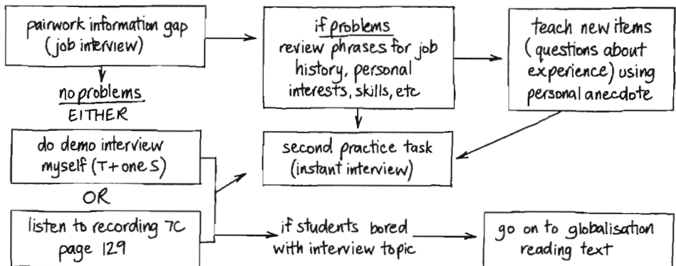
Figure 6.12 Flow chart
